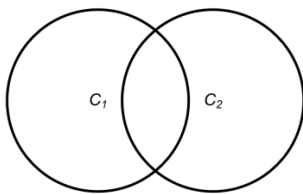
Figure 3. Venn diagram of the set of consequences. The consequences of the event, C_1 , and the final permanent consequences C_2 .
