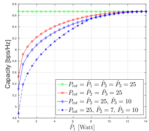
Fig. 1: Capacity under different power constraint settings
