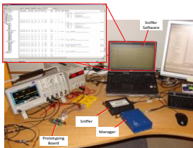
•ABB WirelessHART prototype (2012)
