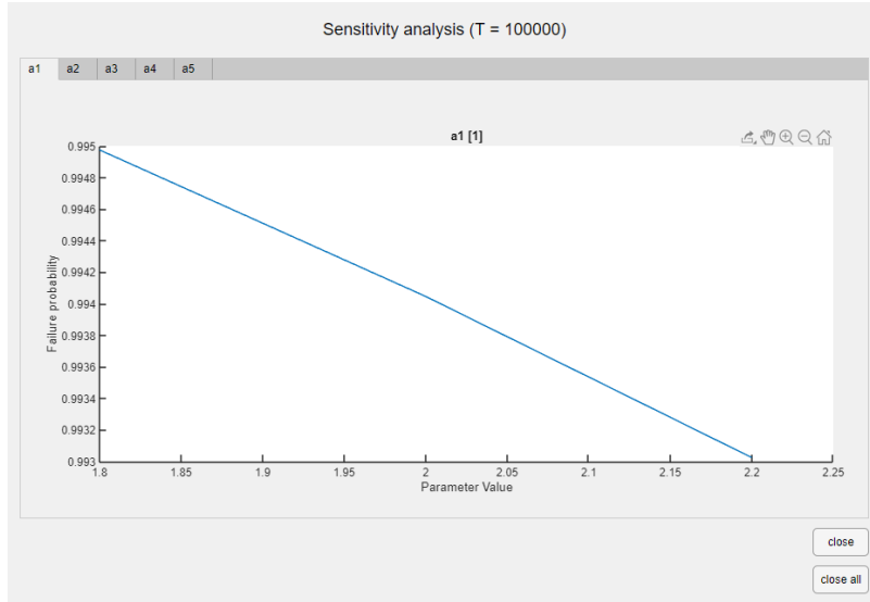
Figure 23: Sensitivity analysis of the modified highway pilot model from figure 21. All parameters have been varied with 10%.
