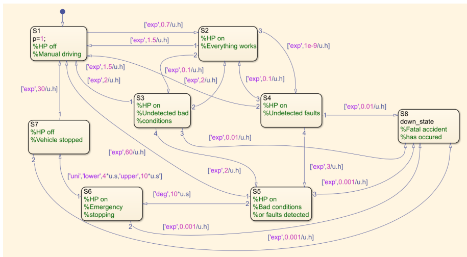
Figure 7: Stateflow model of Highway Pilot, the arcs of the transition arrows have been adjusted for readability after creation.
