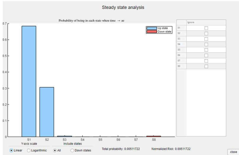
Figure 25: Example simulation of steady state analysis of a slightly modified version of the highway pilot model. Compared to the original version, presented in figure 7, an exponentially distributed transition from S8 to S1 with rate 0.01h has been added.
