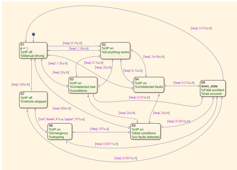
Figure 24: A slightly modified version of the highway pilot model. Compared to the original version, presented in figure 7, an exponentially distributed transition from S8 to S1 with rate 0.01h has been added.
