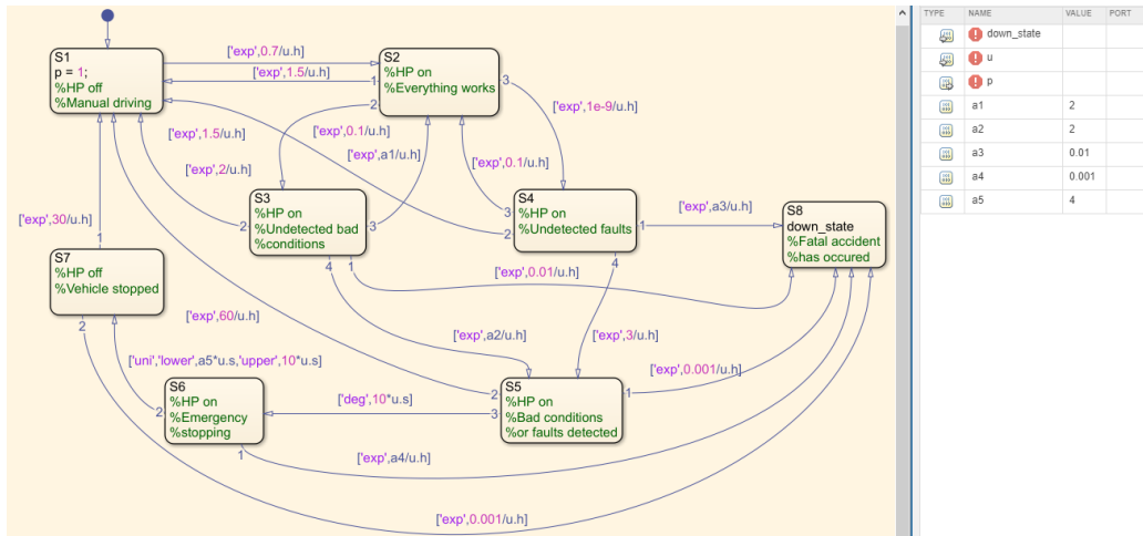
Figure 21: A slightly modified version of the highway pilot model. Compared to the original version, presented in figure 7, some values have been swapped for parameters defined with the same value.
