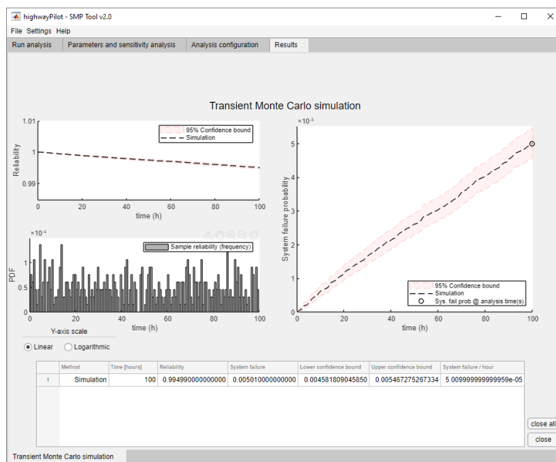
Figure 19: Result from a transient analysis with Monte Carlo simulation of the highway pilot model. The number of simulations used was 100000 and the analysis time was set to 100h.
