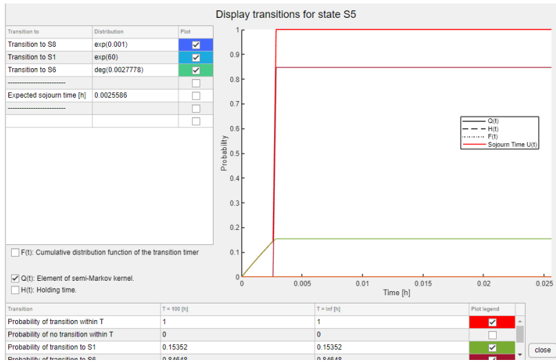
Figure 28: Information window for state S5 of the highway pilot model.
