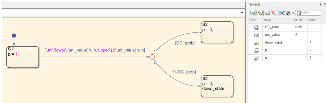
Figure 6: Example model with a branching transition and two specified parameters used to define the branching transition.
