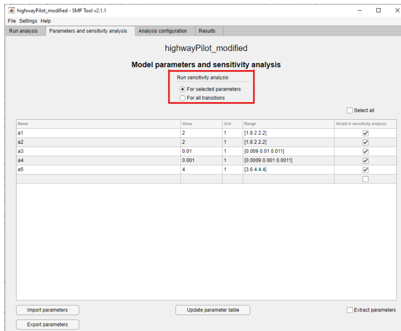
Figure 22: An overview of the settings for sensitivity analysis with a modified version of the highway pilot model.
