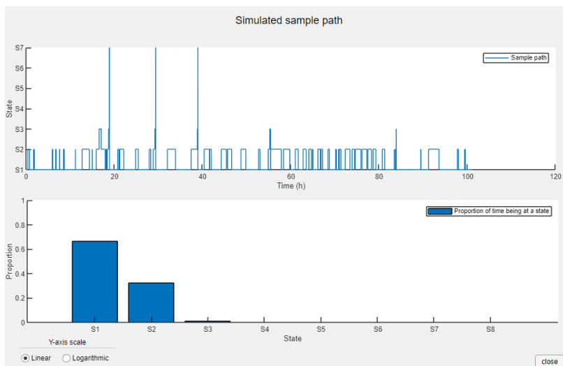
Figure 26: Example simulation of sample path done with the highway pilot model. Analysis time was set to 100h.
