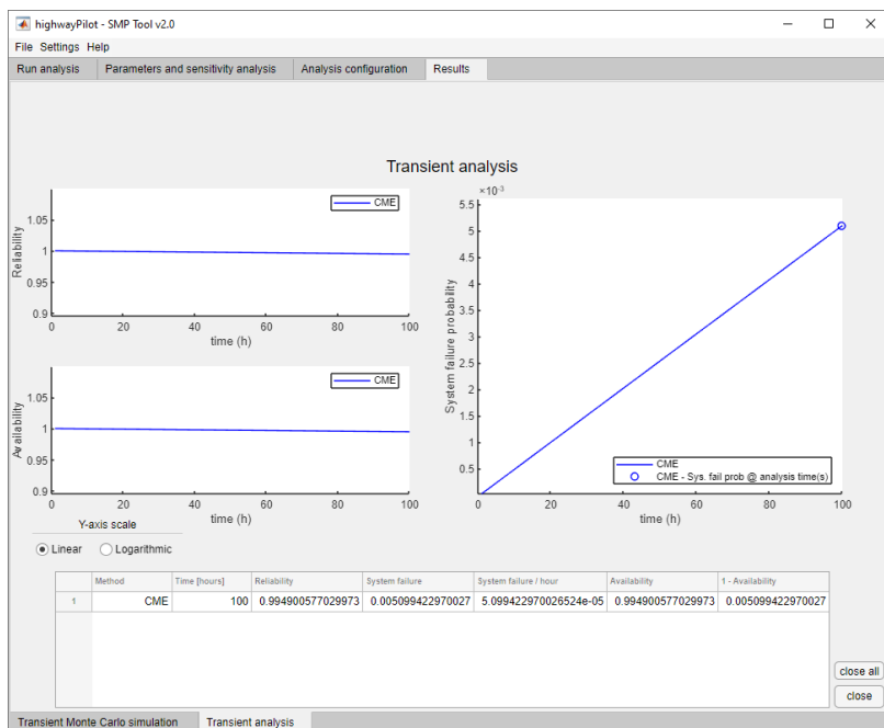
Figure 20: Result from a transient analysis with numerical solver for the highway pilot model. The CME inversion algorithm was used and the analysis time was set to 100h.
