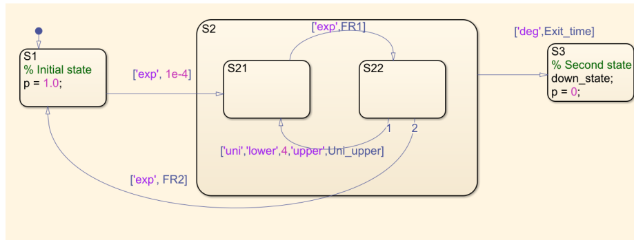
Figure 8: An example HSMP model.
