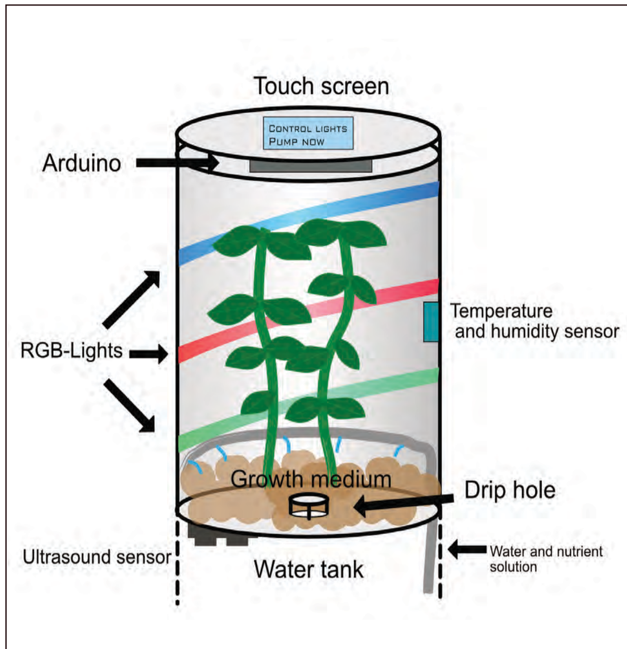
Sketch of the system with components
