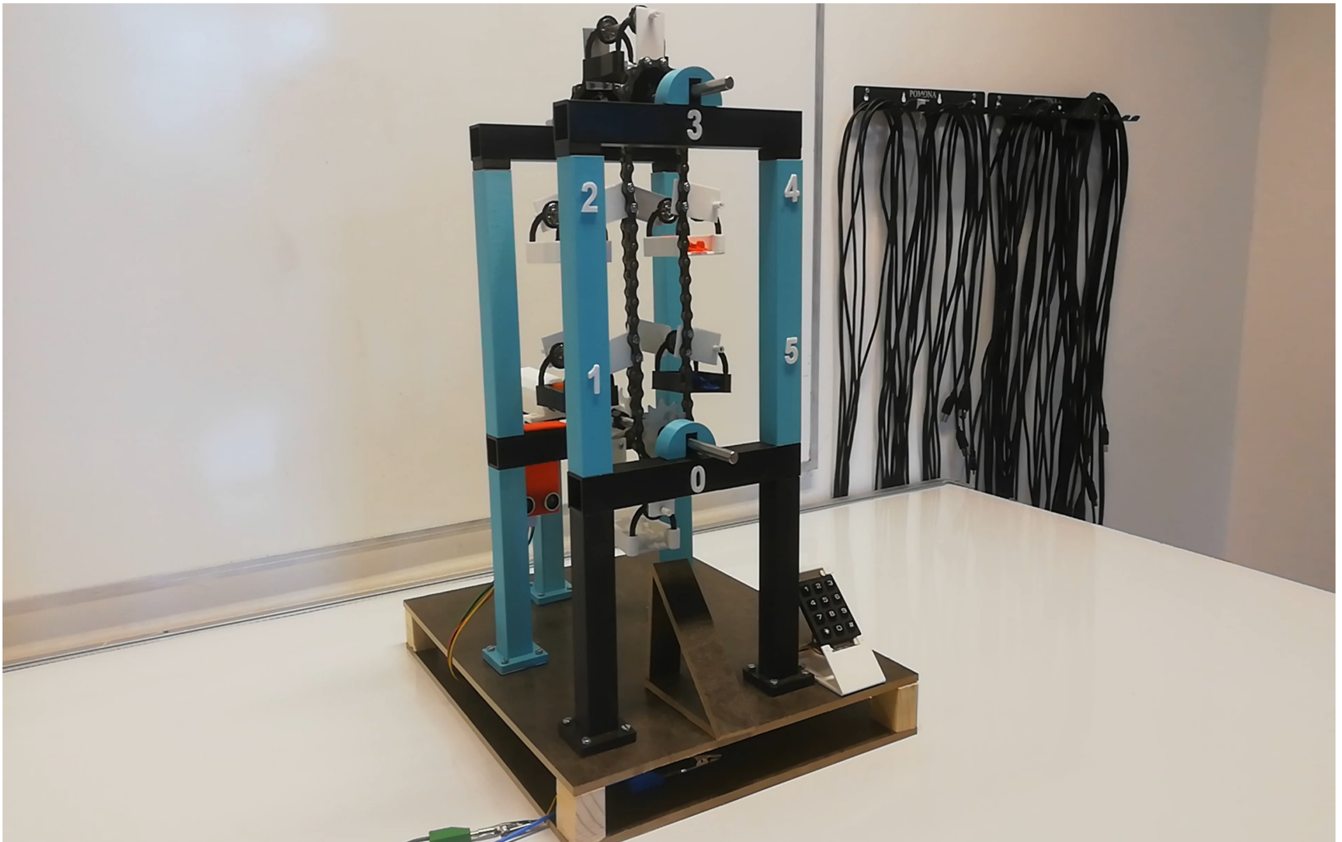
The finished prototype of the rotary parking system.
