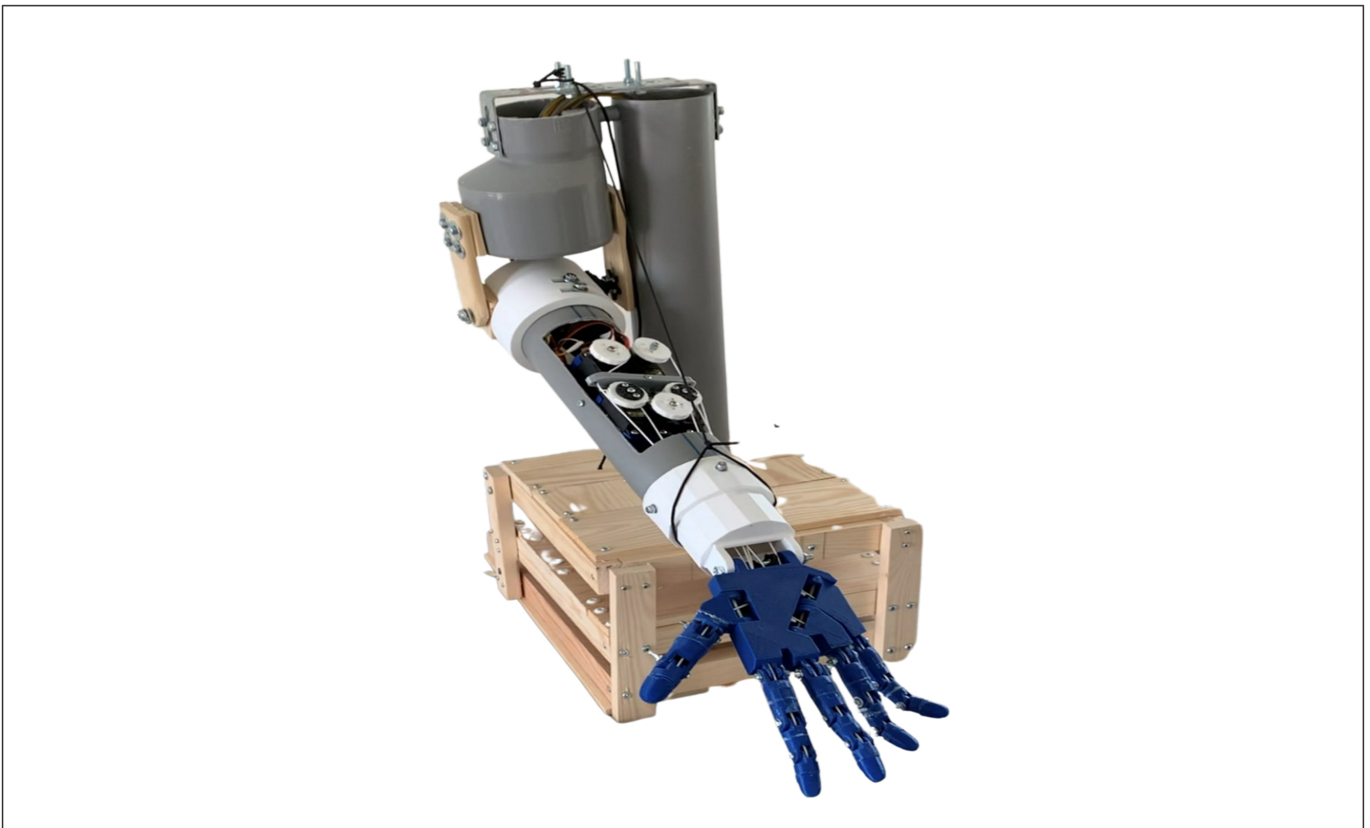
Robotic arm inspired by the human anatomy. It has two degrees of freedom and a flexible grip-function.
