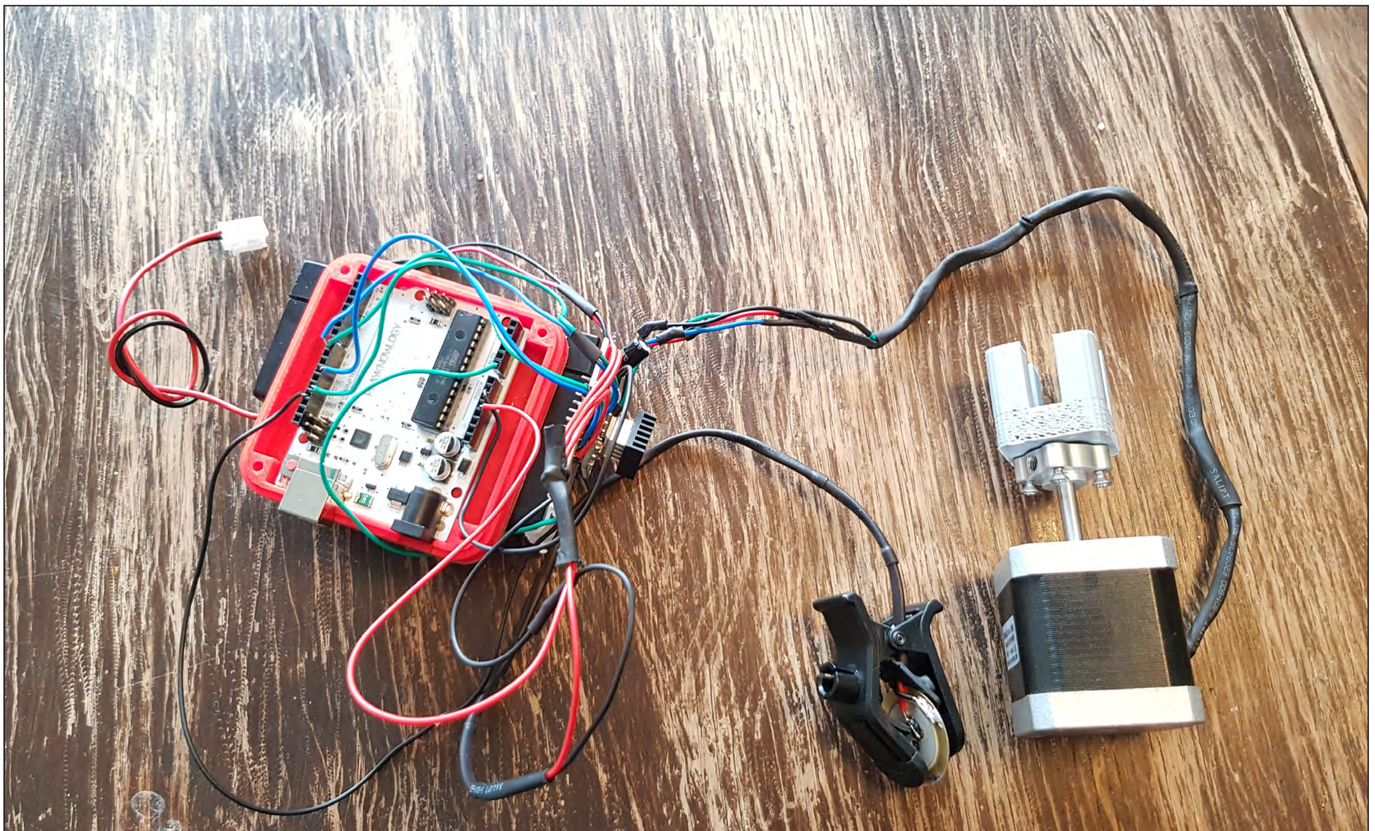
The tuner consists of the Arduino Uno connected to a motor driver and then a stepper motor and a piezoelectric element attached to the clamp in the middle of the picture.
