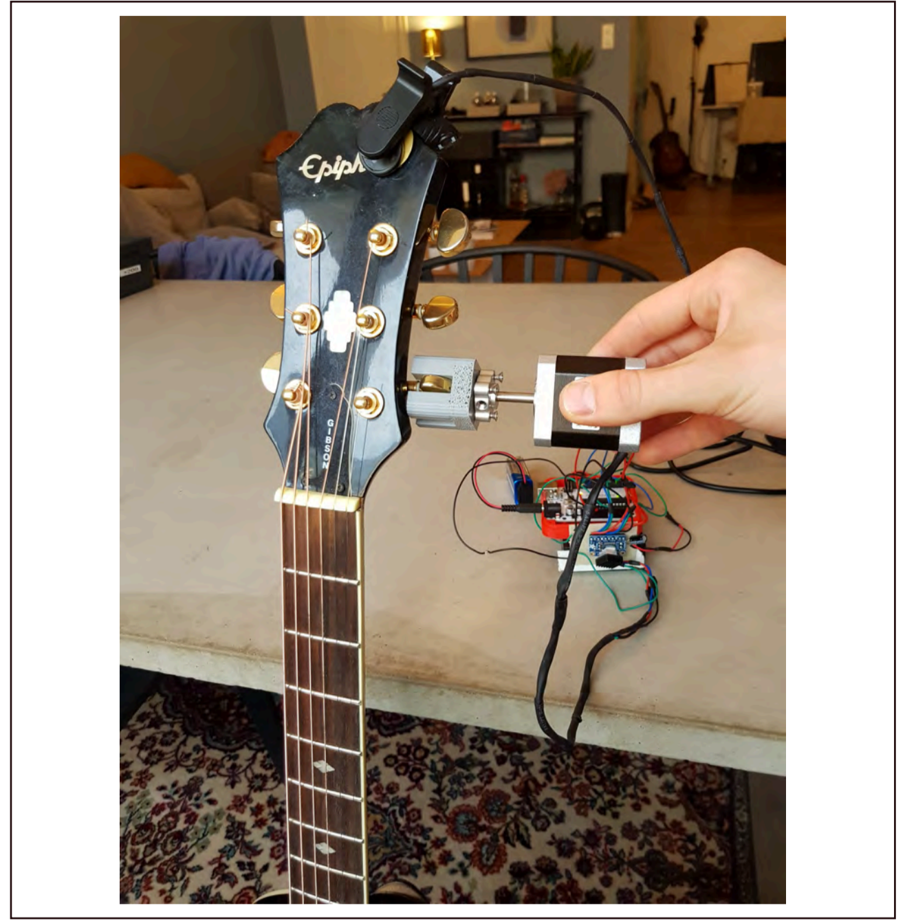
The motor is held at the tuning key corresponding to the string that is being tuned.
