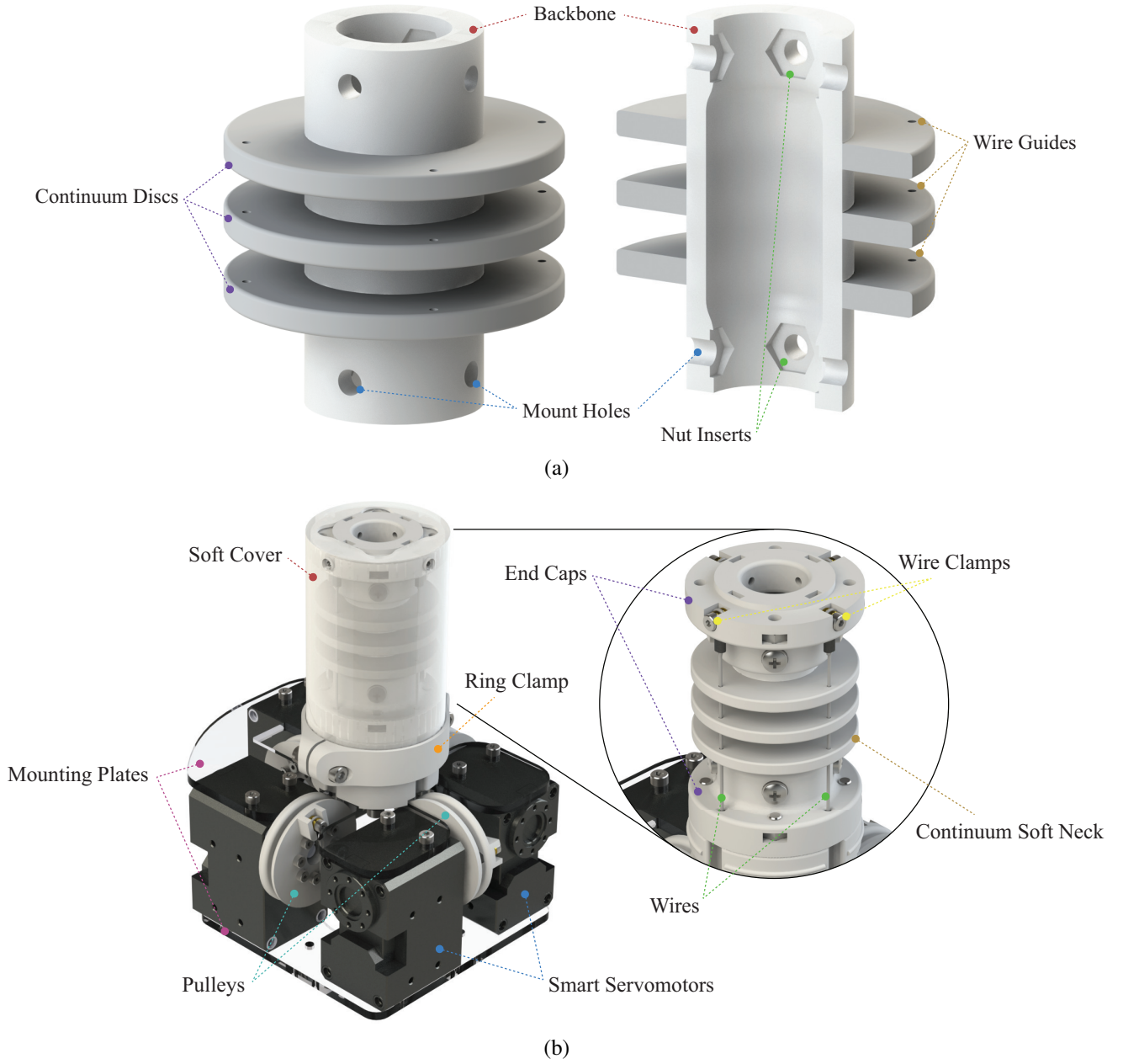
Fig. 2. Graphical representations of the (a) continuum soft neck component in isometric and section view, and (b) soft robotic neck module with annotated main properties.
