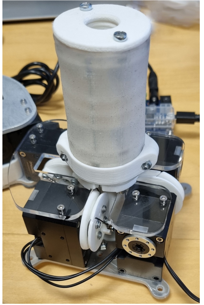
Fig. 3. The assembled robotic neck module prototype.
