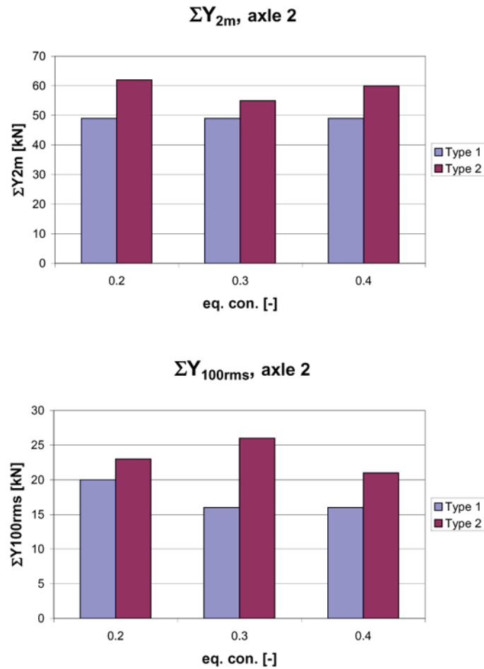
Figure 4-3 \Sigma Y_{2m} (99.85-percentiles) and \Sigma Y_{100rms} for simulations with varying equivalent conicity; 0.2, 0.3 and 0.4, Type 1 and Type 2. Simulations with soft bogie configuration on straight safety track at a vehicle speed of 275 km/h.
