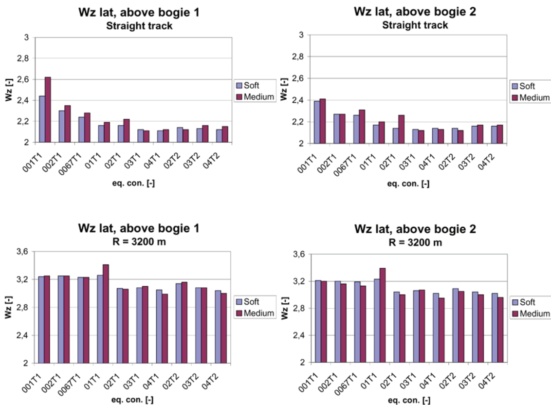
Figure B-3 Lateral W_z on the carbody floor above the two bogies of the soft and medium bogie configurations. Simulations are performed on straight comfort track and in curve with R = 3200 m, at a vehicle speed of 275 km/h. The track plane acceleration is 1.1 \text{ m/s}^2 in the curve.
