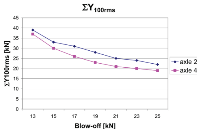
Figure 4-2 Maximum track shift forces ( \Sigma Y_{100rms} ) with varying blow-off level in the yaw dampers. Simulations are performed with soft bogie configuration on straight safety track at a vehicle speed of 275 km/h with equivalent conicity 0.3, Type 2.
