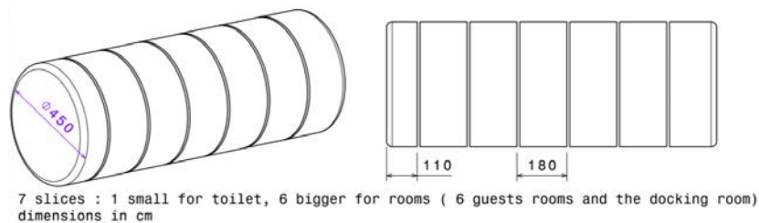
Fig.3 Guest/ Centre Module Layout
