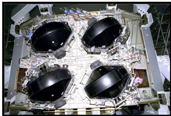
Fig.17 Momentum Wheel
