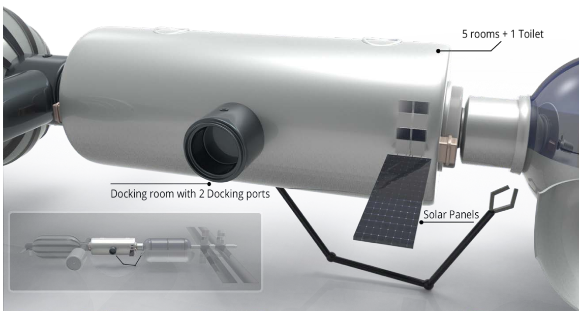
Fig.4 Design of Guest/Centre Module
