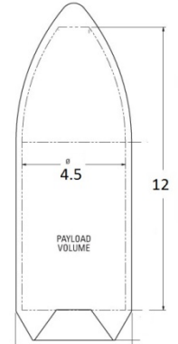
Fig.2 Launcher
