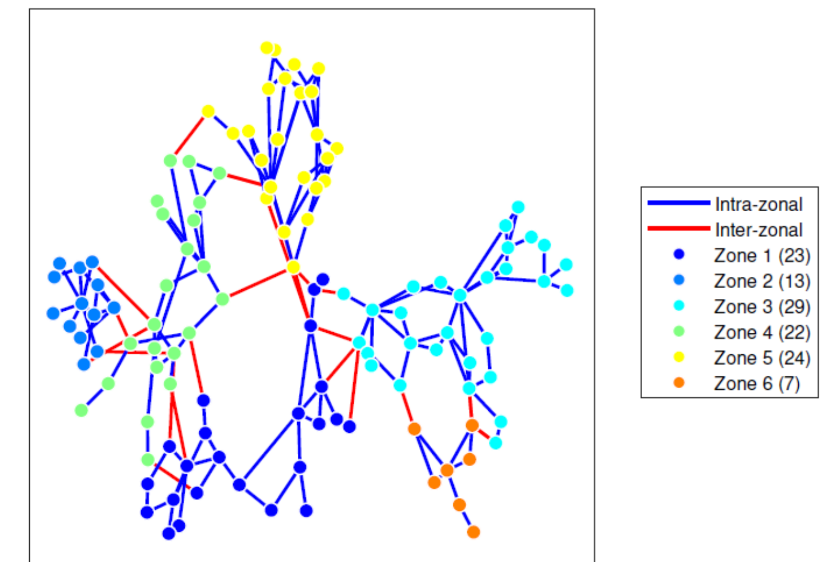
Fig. 1. Cluster example, IEEE 118 bus to 6 zones.
