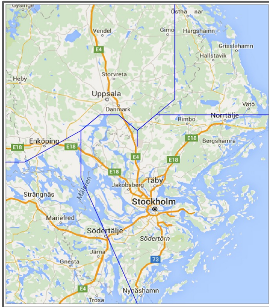
Optimized ground tracks for turned-constrained approaches to Stockholm Arlanda airport
