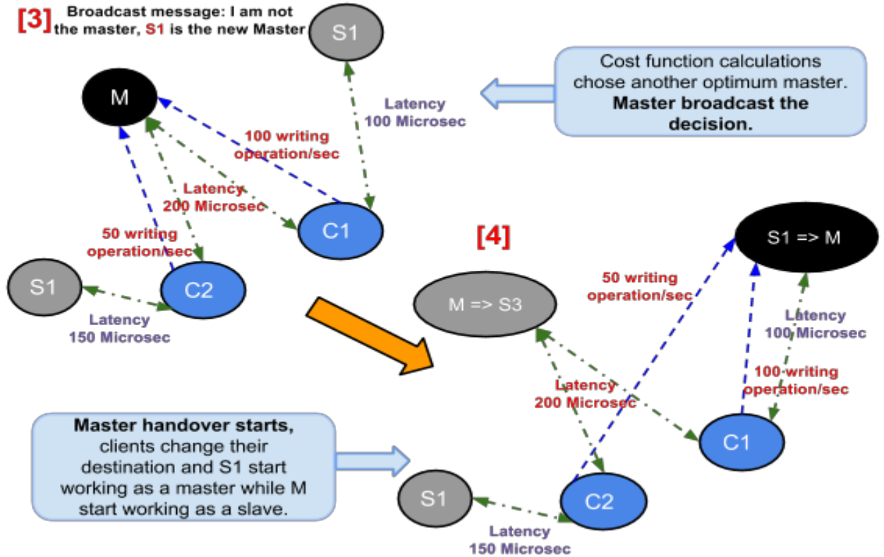
“Figure 7. Master handover state transition”
