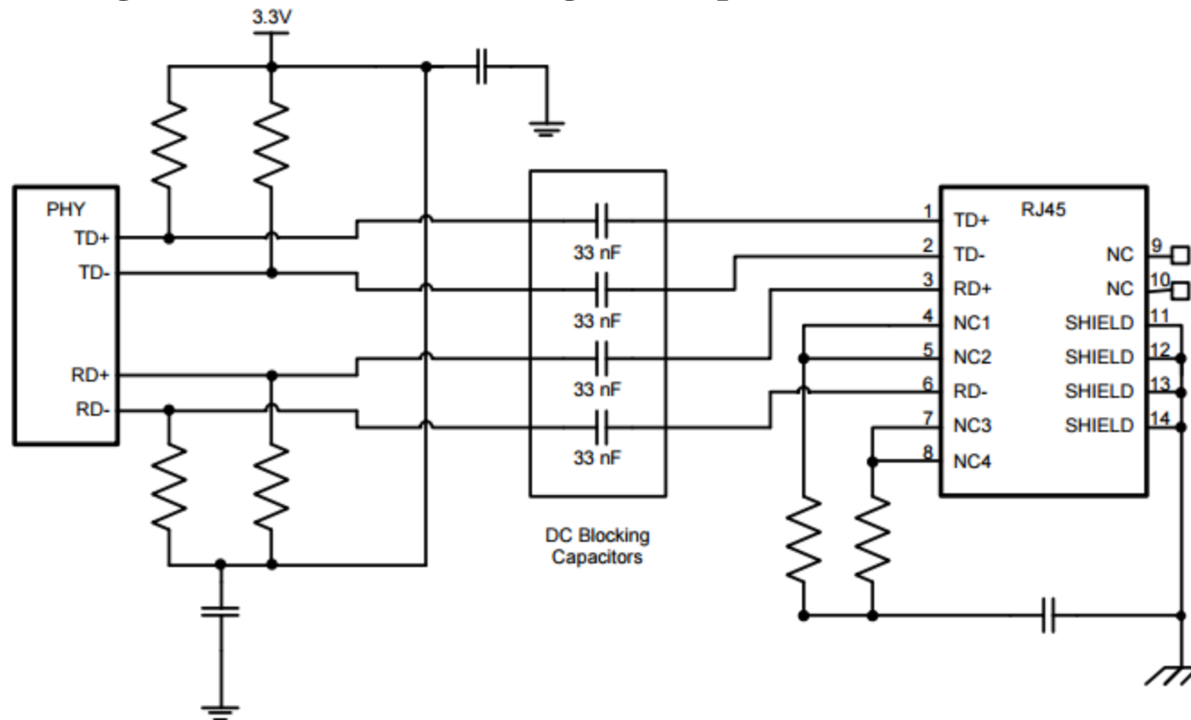
Transformerless Configuration
