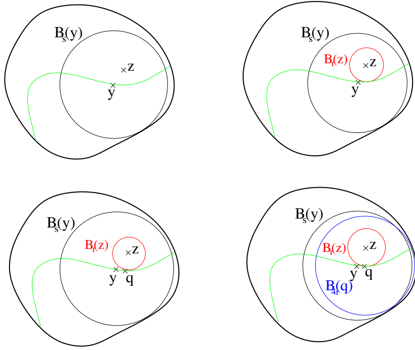
Figure 10: The above figure (not drawn to scale) tries to indicate how B_r(z) and B_{4r}(q) is chosen. We have the point y such that B_s(y) \subset D shown in the first figure. The ball B_r(z) (in red) is then chosen to be the largest ball contained in \Omega = \{u > 0\} . That means that \partial B_r(z) touches the free boundary (the green curve) in some point q as shown in the third picture. We then choose the ball B_{4r}(q) (in blue) as in the last picture. The purpose of this construction is that since B_{4r}(q) \subset D we know, Theorem 5.1, that u(x) is uniformly bounded in B_r(z) \subset B_{4r}(q) .
