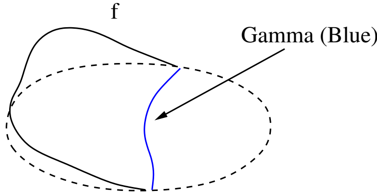
Figure 7: The graph of a typical solution to the normalized obstacle problem in the ball. The graph takes the values f(x) on the boundary. The solution
