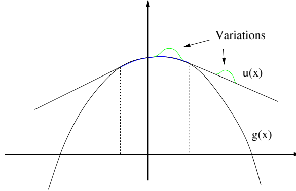
Figure 6: A graphical representation of the variations, if the bump \phi is added in a region where u(x) = g(x) (as in the left bump in the graph) then we get the inequality (36). But if the bump is added away from the touching set (as the right bump) then we may do variations with t \in (-\epsilon, \epsilon) and thus get the full equality as in (37).
