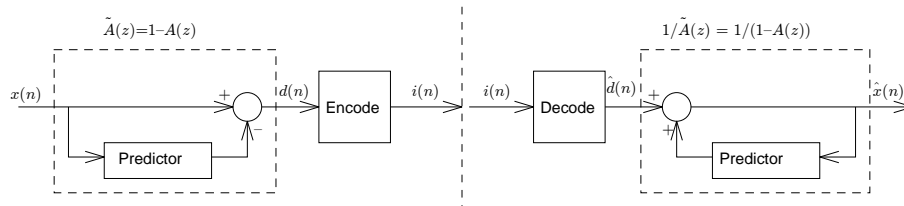
Figure 1: Open loop DPCM (adaptation not illustrated)
