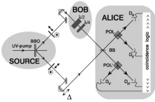
FIG. 1. Experimental setup for quantum dense coding. Because of the nature of the Si-avalanche photodiodes, the extension shown in the inset of Fig. 4 is necessary for identifying two-photon states in one of the outputs.
