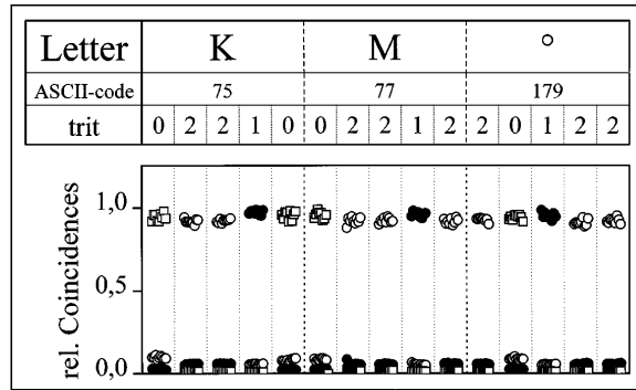
FIG. 5. "1.58 bit per photon" quantum dense coding: The ASCII codes for the letters "KM o " (i.e., 75, 77, 179) are encoded in 15 trits (with "0" \equiv |\Phi^-\rangle \hat{=} \square , "1" \equiv |\Psi^+\rangle \hat{=} \bullet , and "2" \equiv |\Psi^-\rangle \hat{=} \circ ) instead of the 24 bits usually necessary. The data for each type of encoded state are normalized to the maximum coincidence rate for that state.
