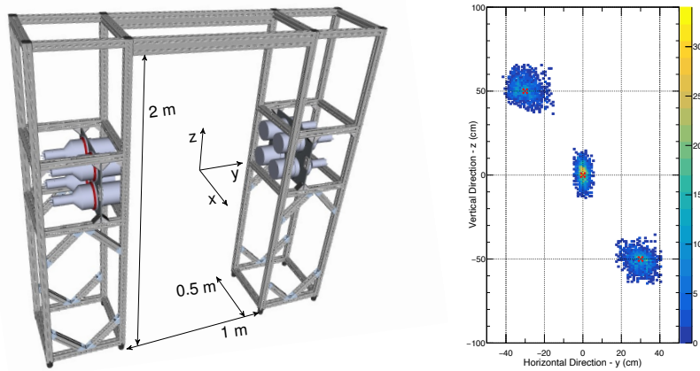
Fig. 1. Left: CAD model of the prototype RPM system including its mechanical support structure. Right: Results of repeated measurements for three different placements of a 3.2 \cdot 10^{-9} g encapsulated Cf-252 spontaneous fission source. See Ref. 3) for details. 7
