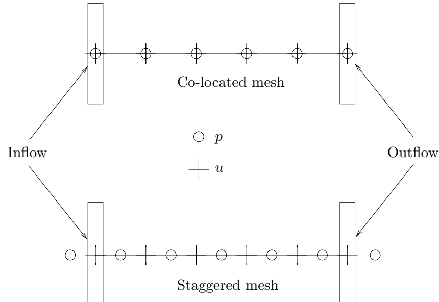
Figure 1: Schematics of a co-located and a staggered grid, respectively.
