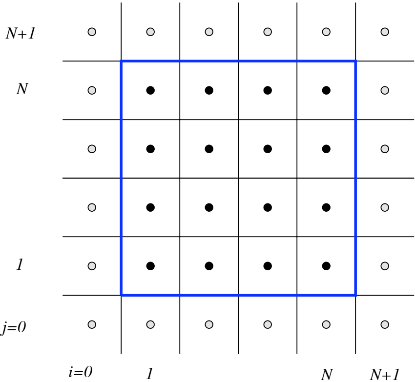
Figure 1: Sketch of the grid. Black dots denote the (N \times N) positions in which the pressure is evaluated, whereas gray dots indicate dummy cells situated outside the computational domain.
