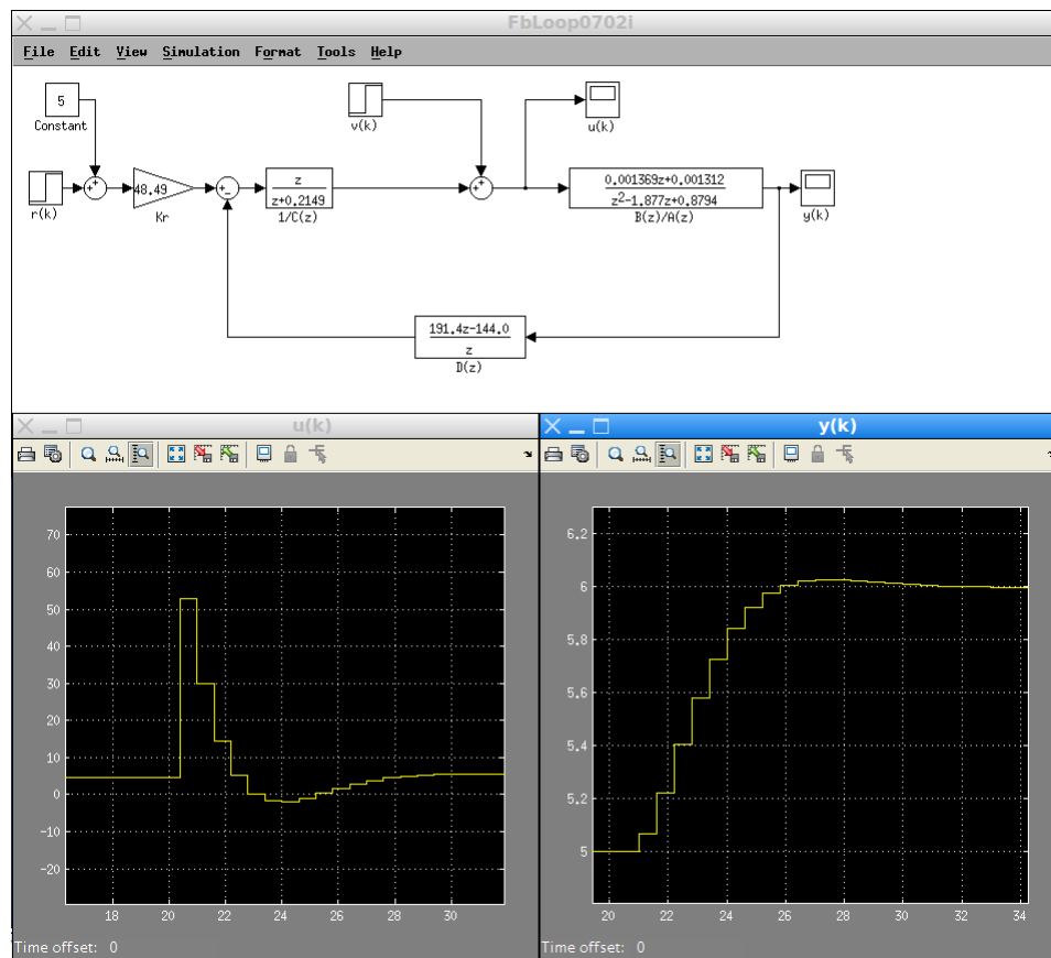
Figure 2: Simulation of reference value step from 5 to 6. There is no disturbance, v(k) = 0 . HP = \frac{0.001369z^{-1}+0.001312z^{-2}}{1-1.877z^{-1}+0.8794z^{-2}} , poles in z = 0.7 \pm 0.2i
