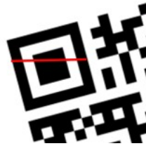
FIGURE 3.1: Row Scanning
