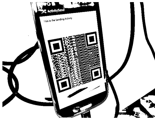
(b) Thresholding
