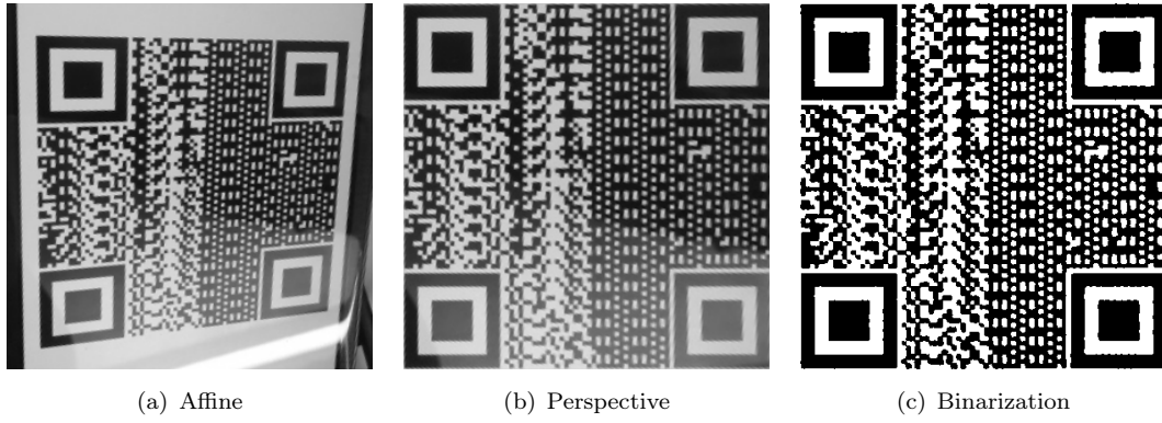
FIGURE 3.11: Image Transformation
