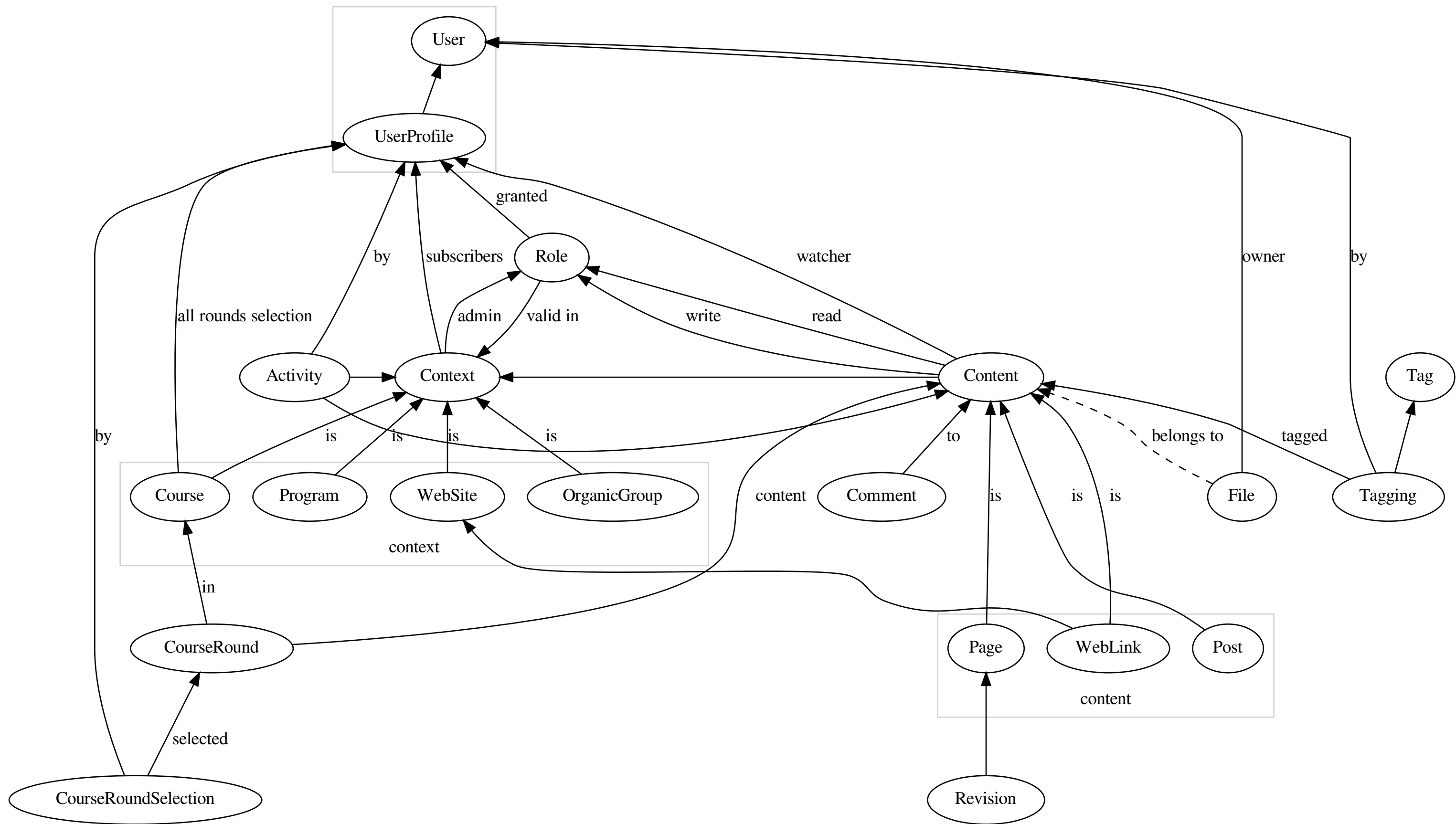
Domain Model
